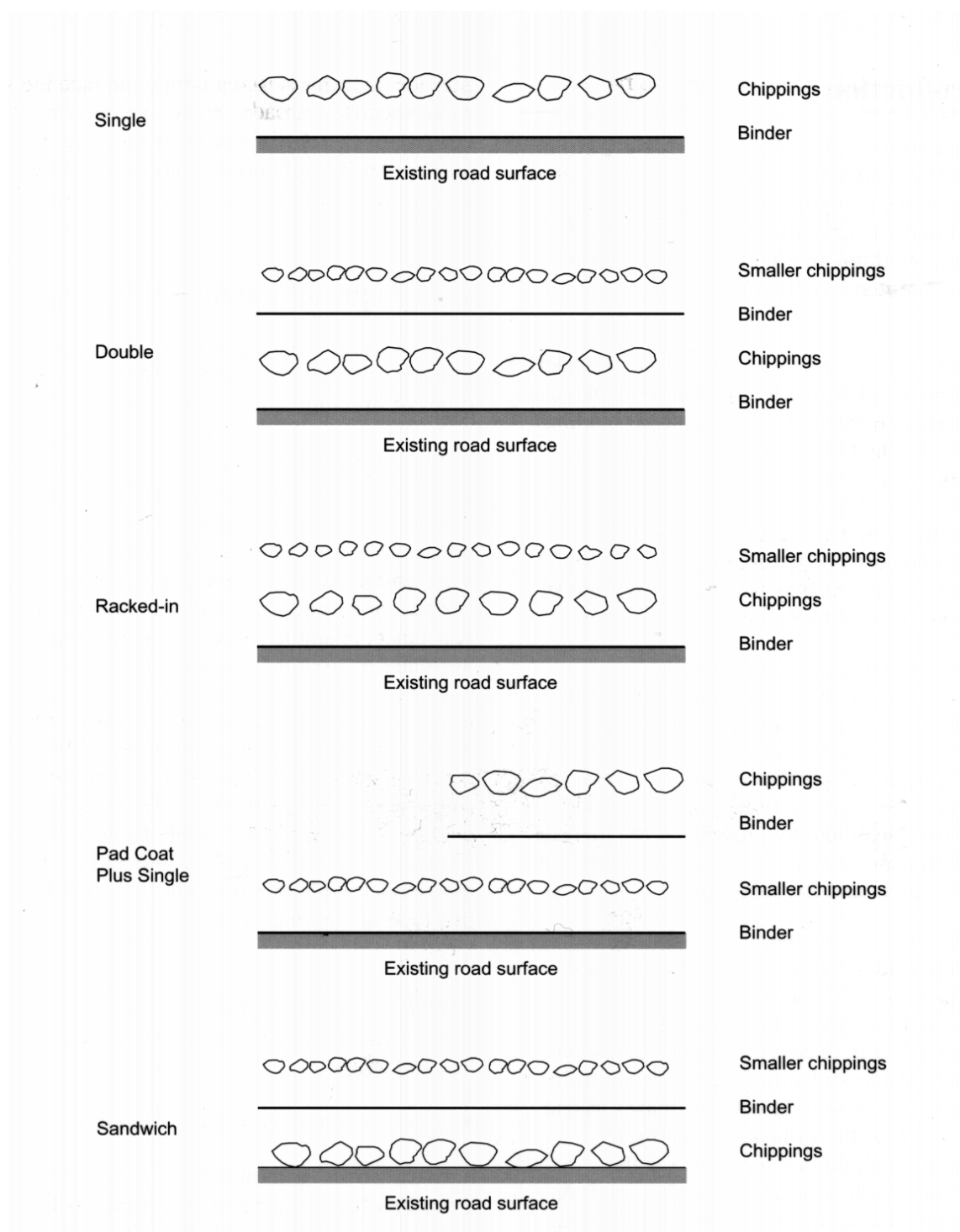
Figure 1 Type of surface dressings
